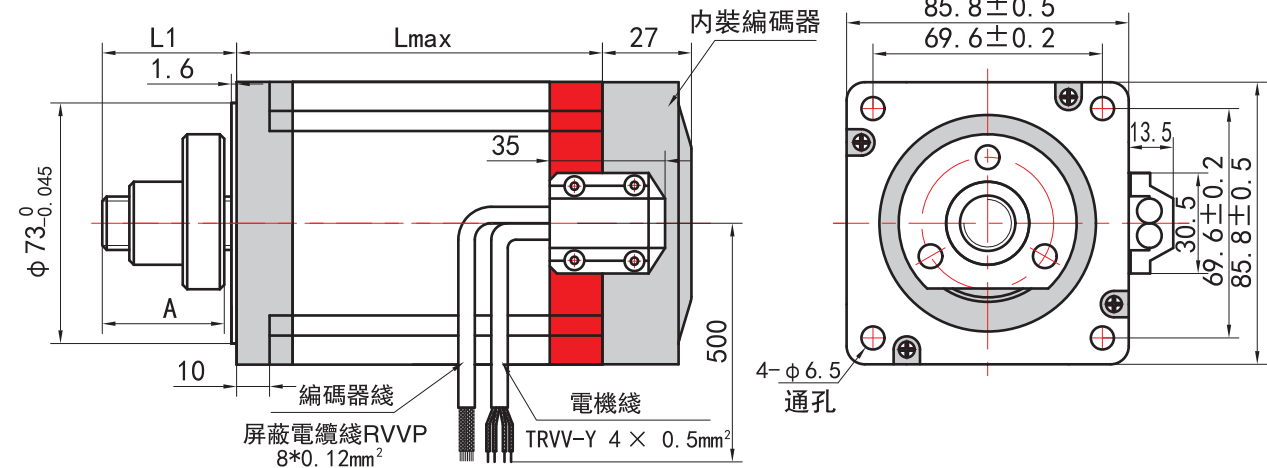
34HS-LExx-E 集成编码器 With encoder
