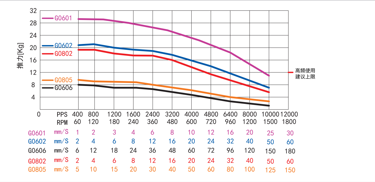
Force-Velocity Curve-14HS34
