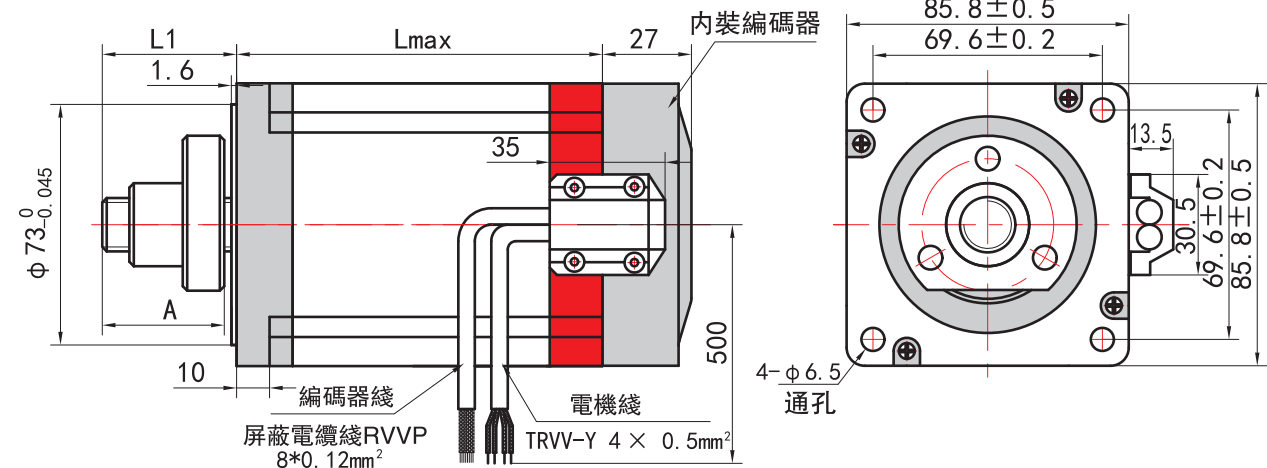
34HS-LExx-BE17 集成多圈绝对值编码器 With Multi-Turn Absolute Encoder
