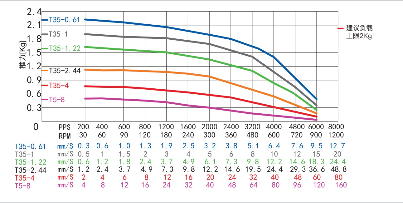
Force-Velocity Curve-8HY30
