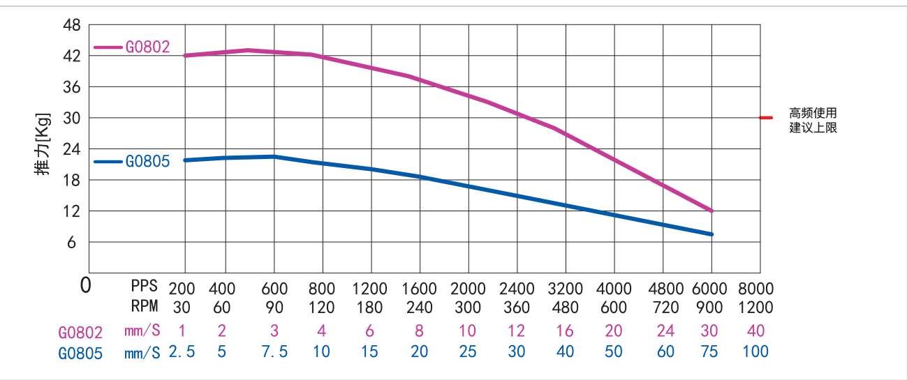
Force-Velocity Curve-17HS48
