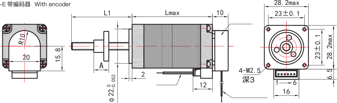
11HY-LExx-E 带编码器 With encoder
