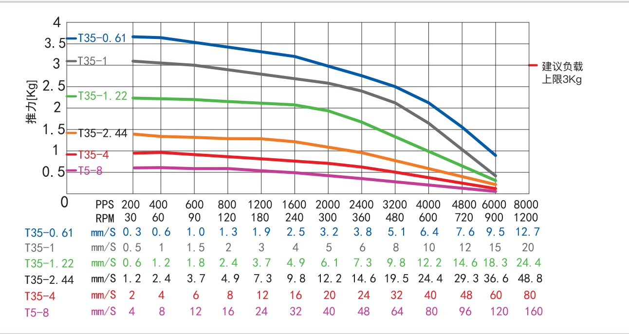
Force-Velocity Curve-8HY38
