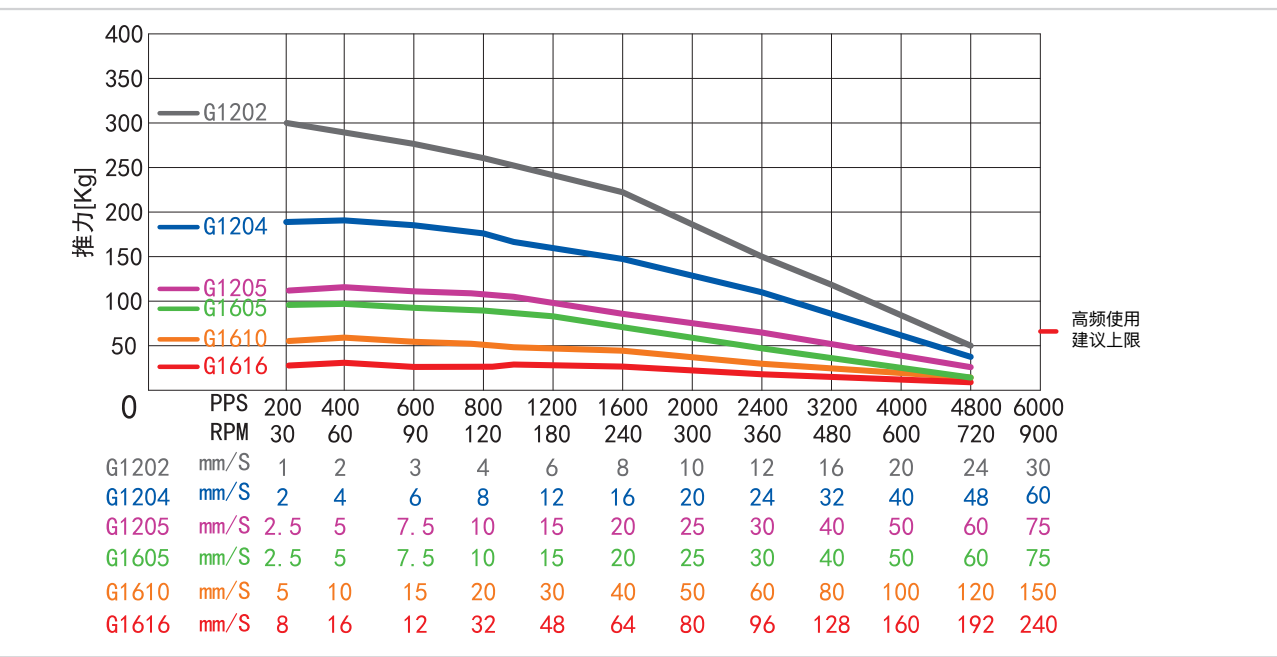
Force-Velocity Curve-23HS76
