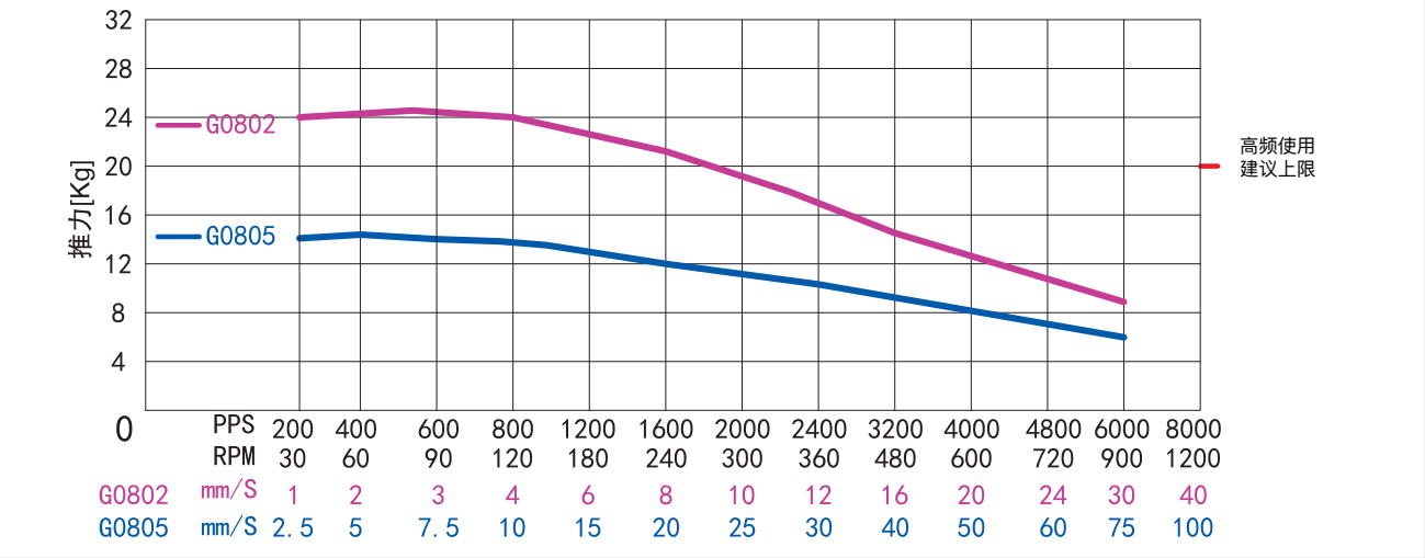
Force-Velocity Curve-17HS34
