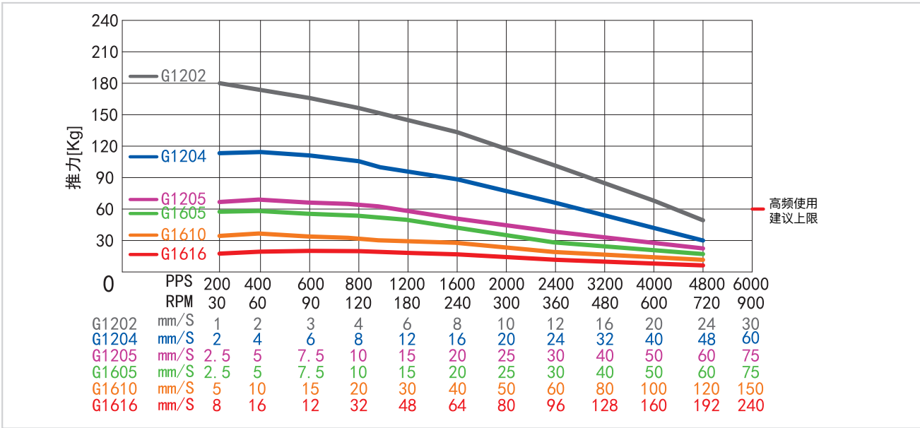
Force-Velocity Curve-23HS56
