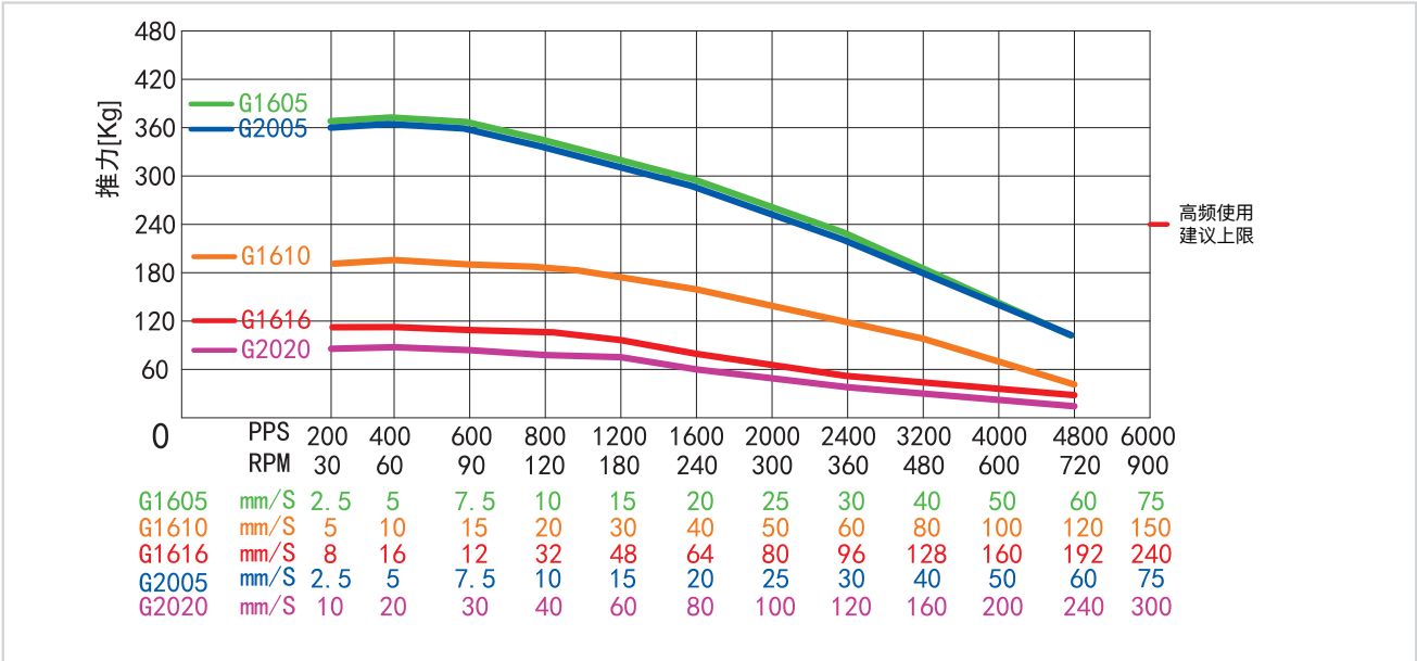
Force–Velocity Curve–34HS98
