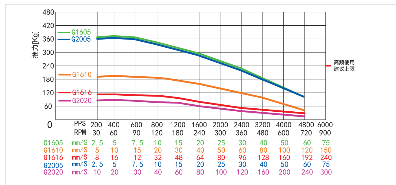
Force-Velocity Curve-34HS98
