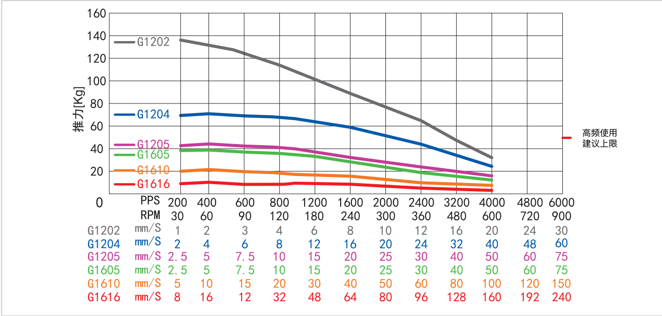
Force-Velocity Curve-23HS45
