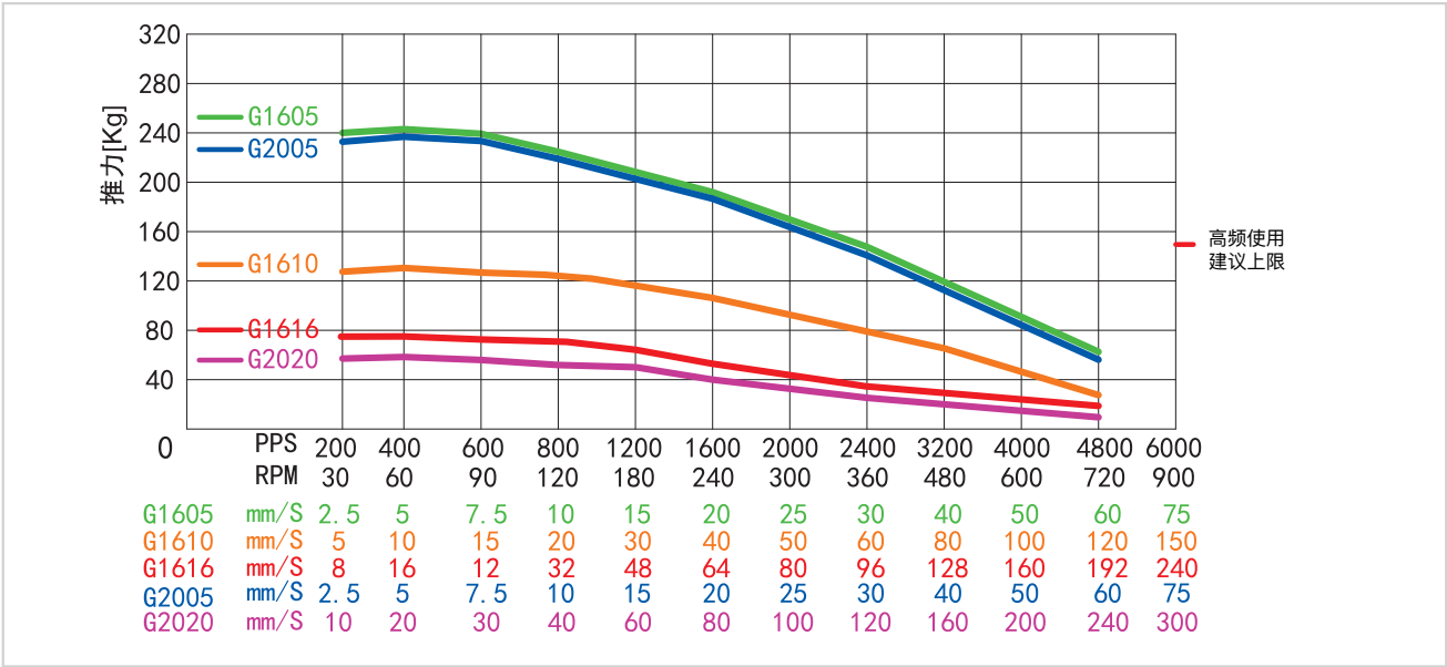
Force–Velocity Curve–34HS76
