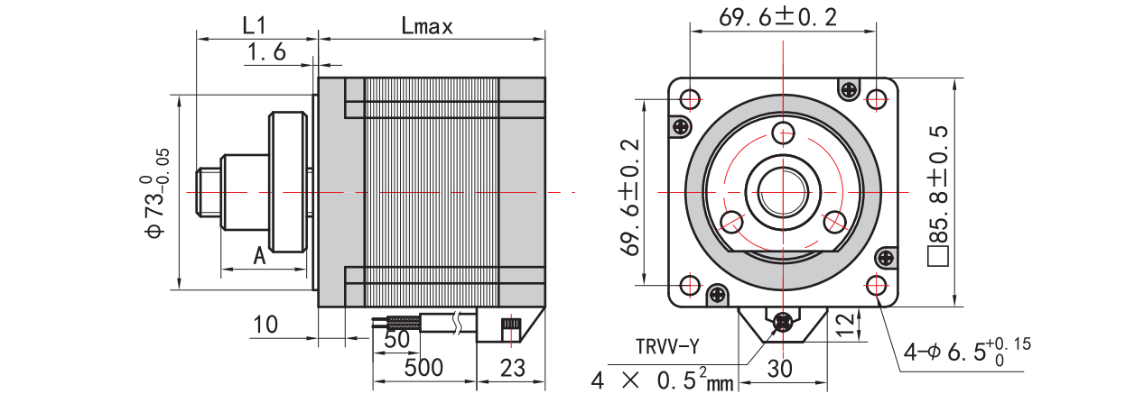
34HS01-LExx 无编码器 Without encoder
