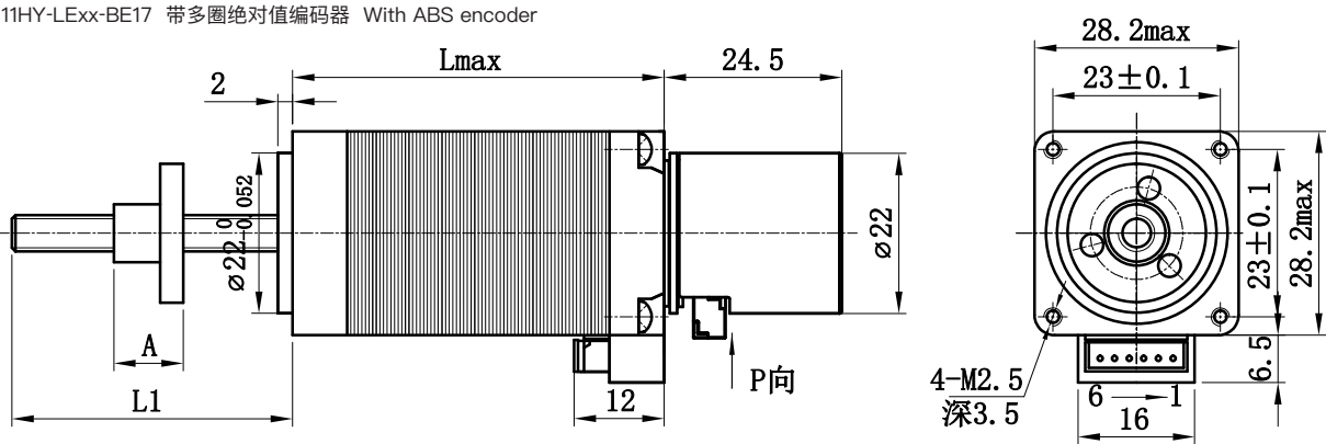
11HY-LExx-BE17 带多圈绝对值编码器 With ABS encoder
