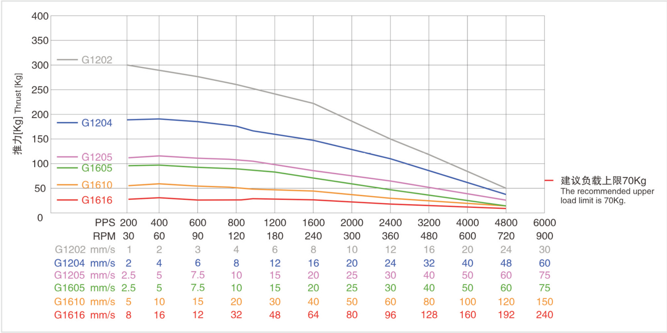
Force–Velocity Curve–23HS76
